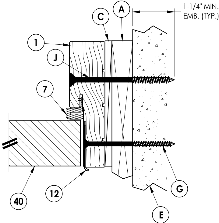
2 HORIZONTAL CROSS SECTION 4 Inswing Shown 1X Buck Construction
