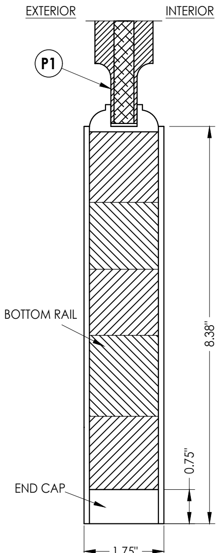
4 2 VERTICAL CROSS SECTION
