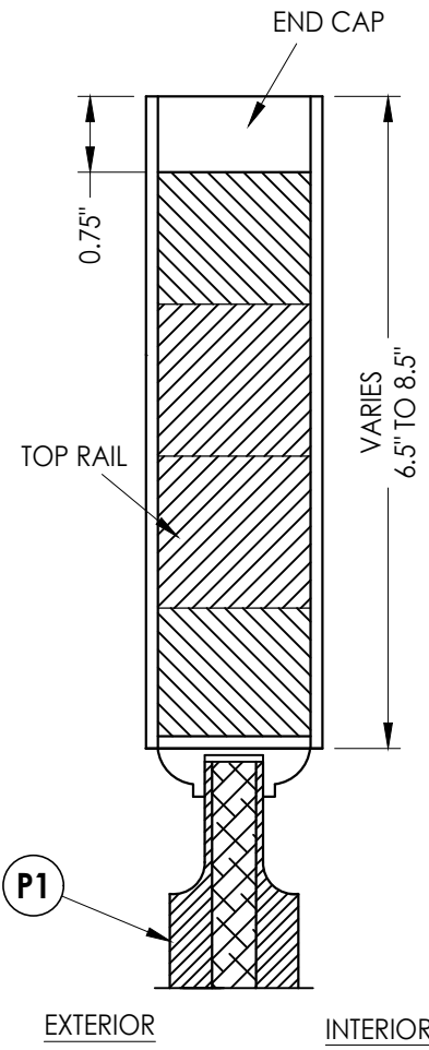
2 2 VERTICAL CROSS SECTION
