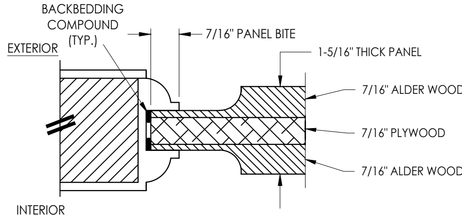
P1 PANEL DETAIL DOOR
