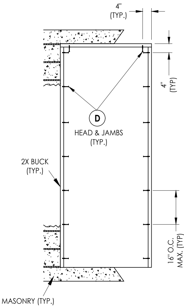
2X BUCK ANCHORING
