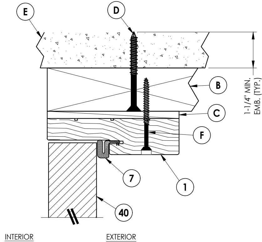
3 3 VERTICAL CROSS SECTION Inswing Shown 2X Buck Construction
