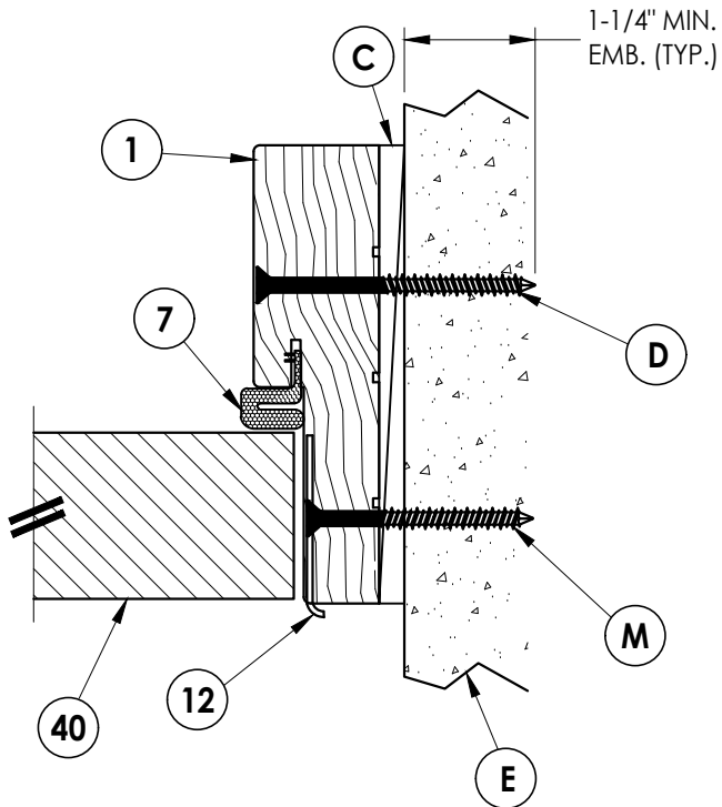
2 HORIZONTAL CROSS SECTION 5 Inswing Shown Shown Direct to Masonry
