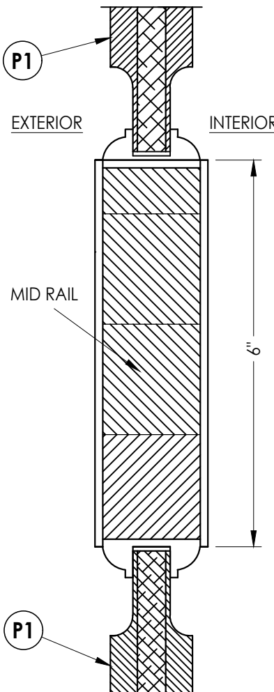
3 2 VERTICAL CROSS SECTION
