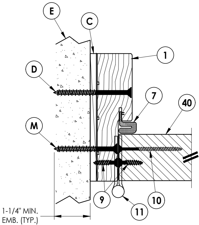
1 HORIZONTAL CROSS SECTION 5 Inswing Shown Shown Direct to Masonry
