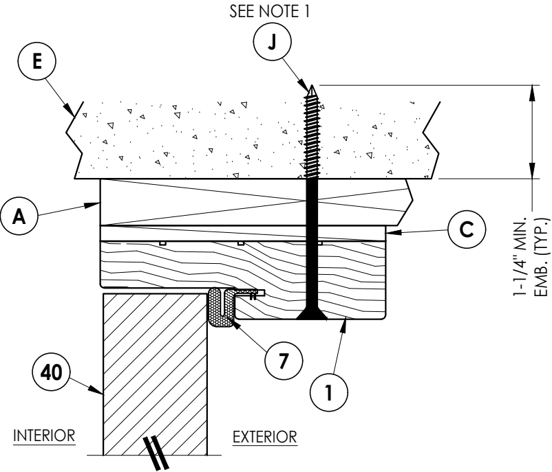
3 VERTICAL CROSS SECTION 4 Inswing Shown 1X Buck Construction
