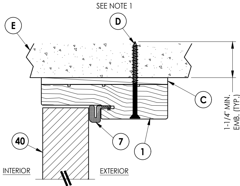
3 VERTICAL CROSS SECTION 5 Inswing Shown Shown Direct to Masonry
