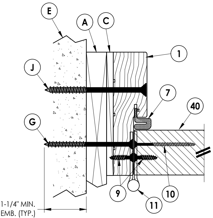
1 HORIZONTAL CROSS SECTION 4 Inswing Shown 1X Buck Construction
