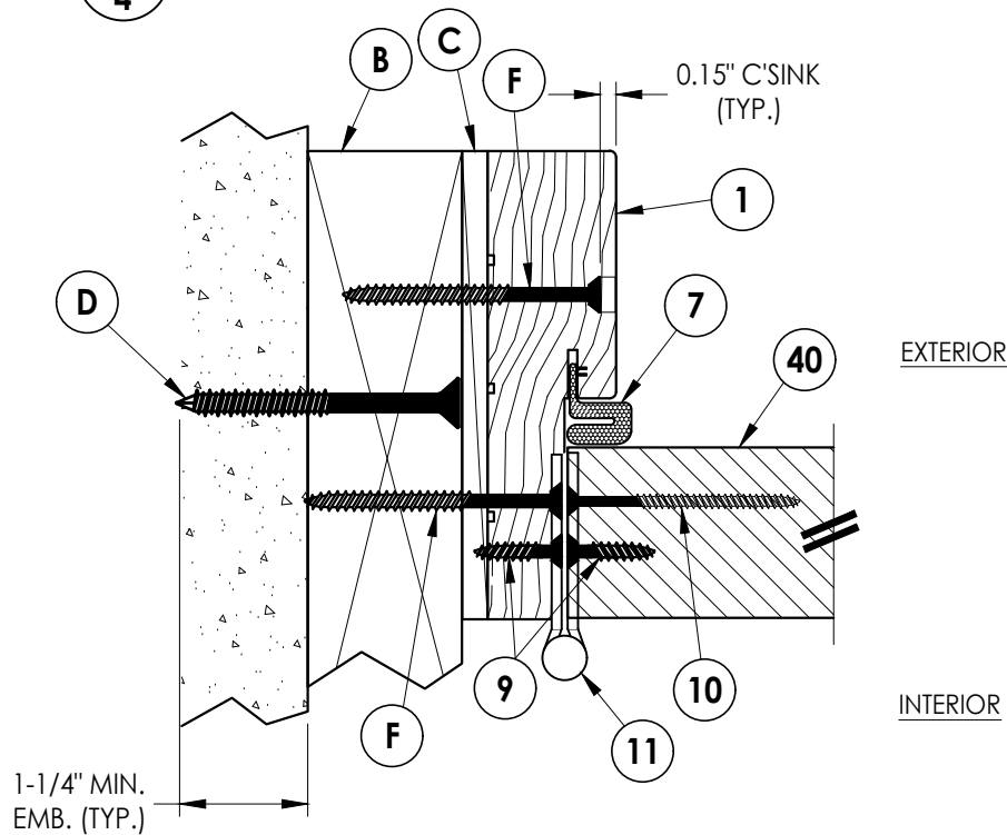
1 3 HORIZONTAL CROSS SECTION Inswing Shown 2X Buck Construction
